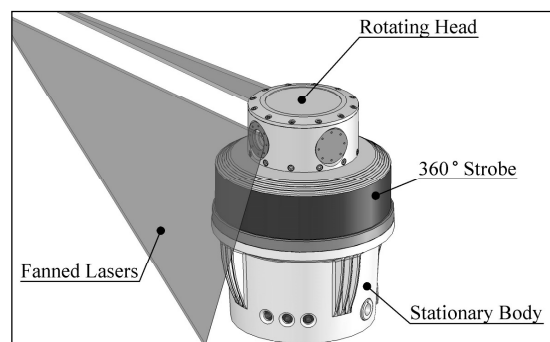
Fig. 2 - Main Components of iGPS Transmitter
