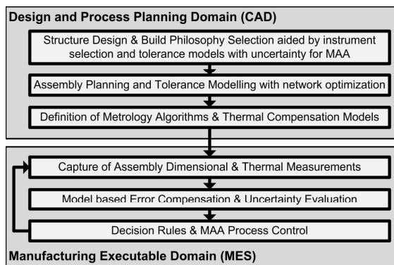
Fig. 5. Summary of Integrated Dimensional Variation Management
