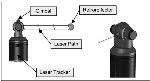
Fig. 1 – Laser Tracker Operation
